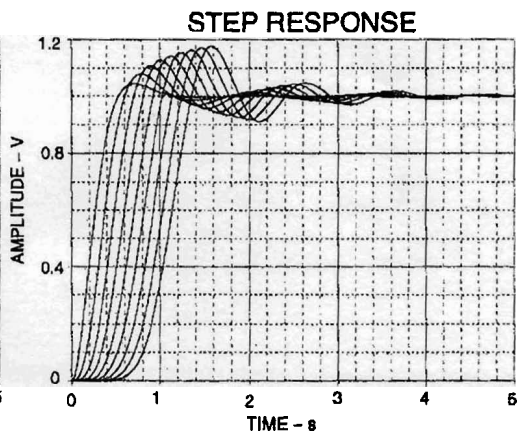
Figure 5-15: Butterworth response
