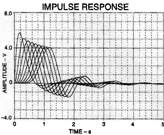
Figure 5-15: Butterworth response
